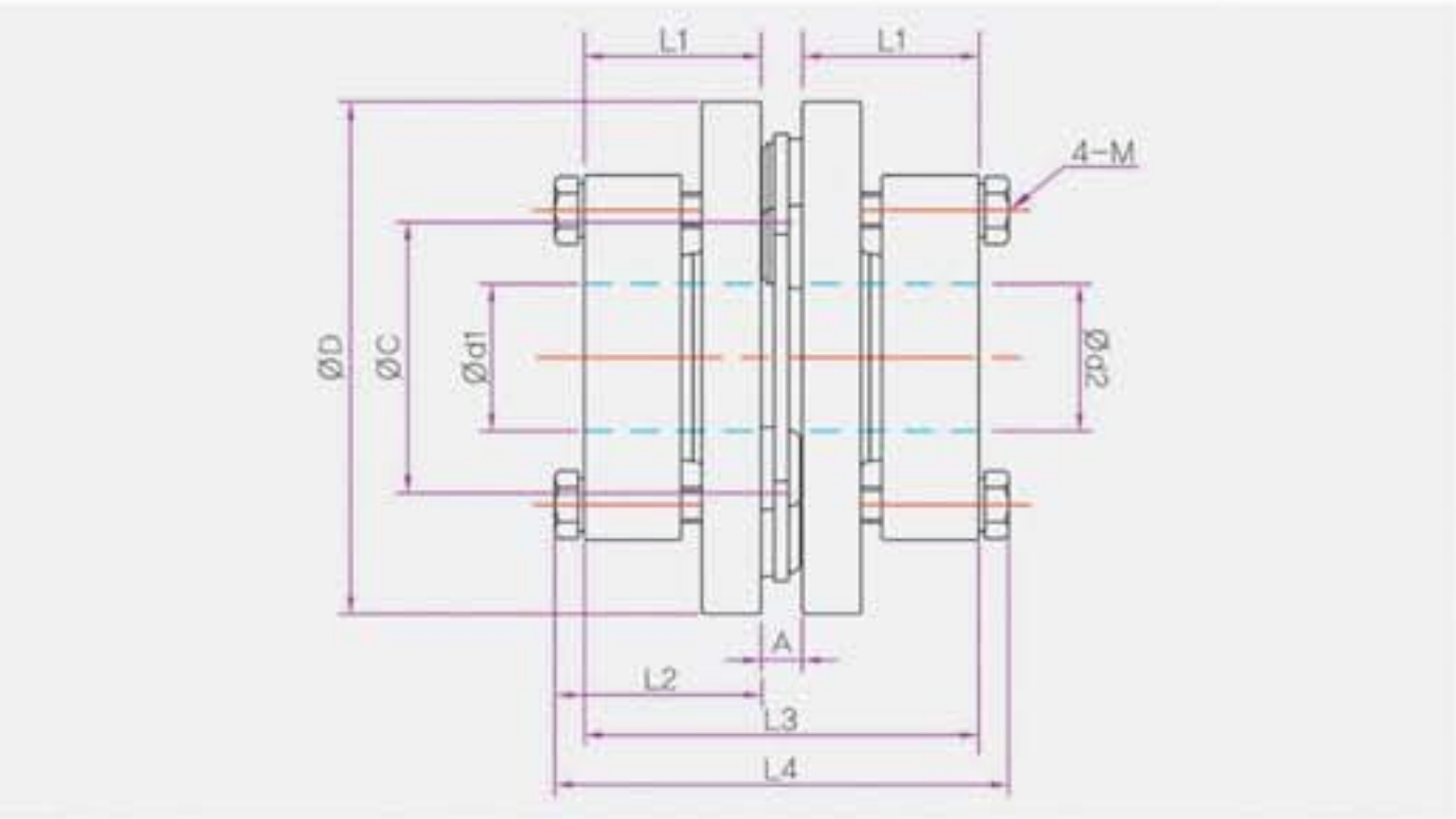
SHDS - ■■■T (TAPER TYPE)
