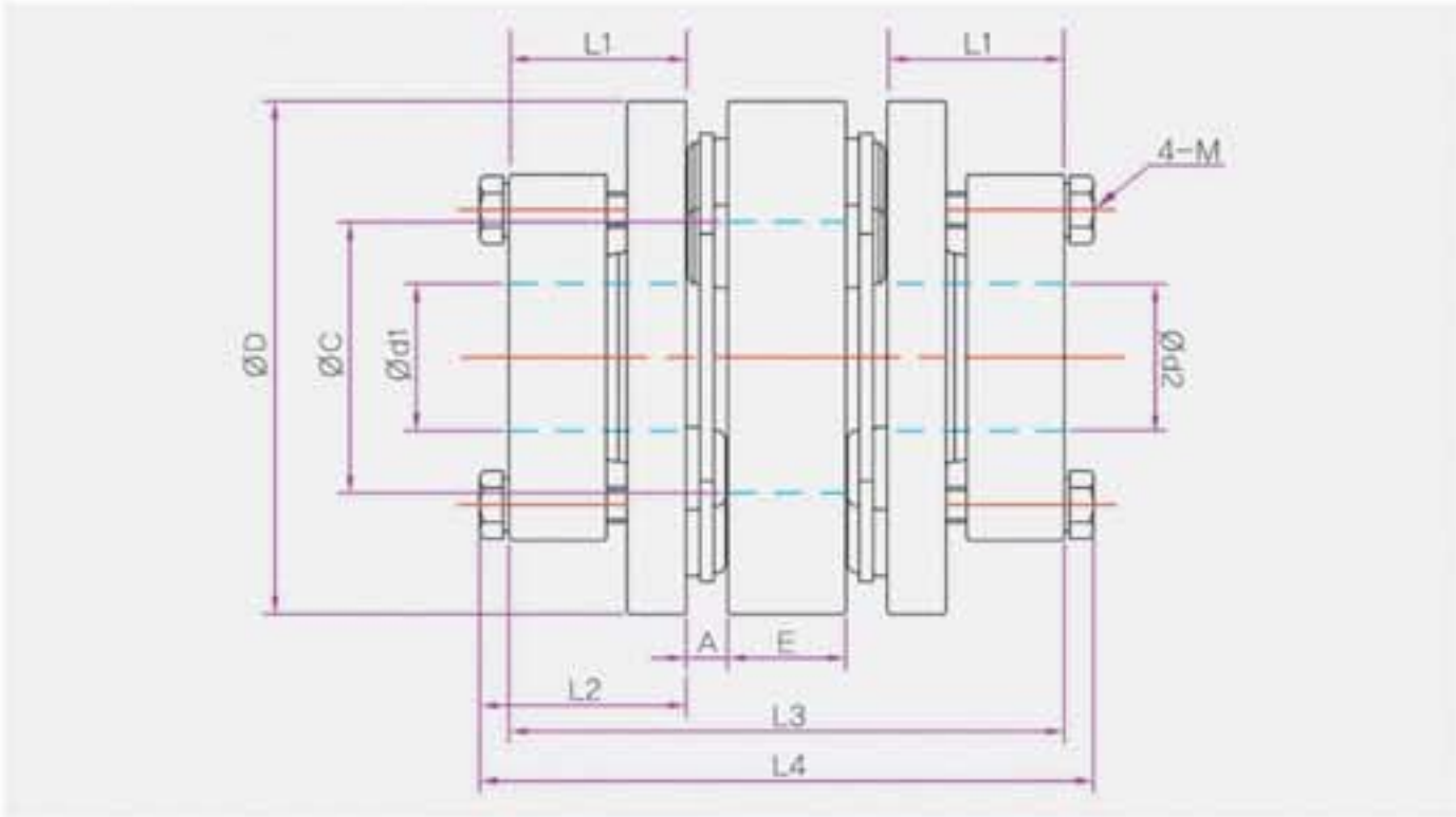
SHDW - ■■■T (TAPER TYPE)
