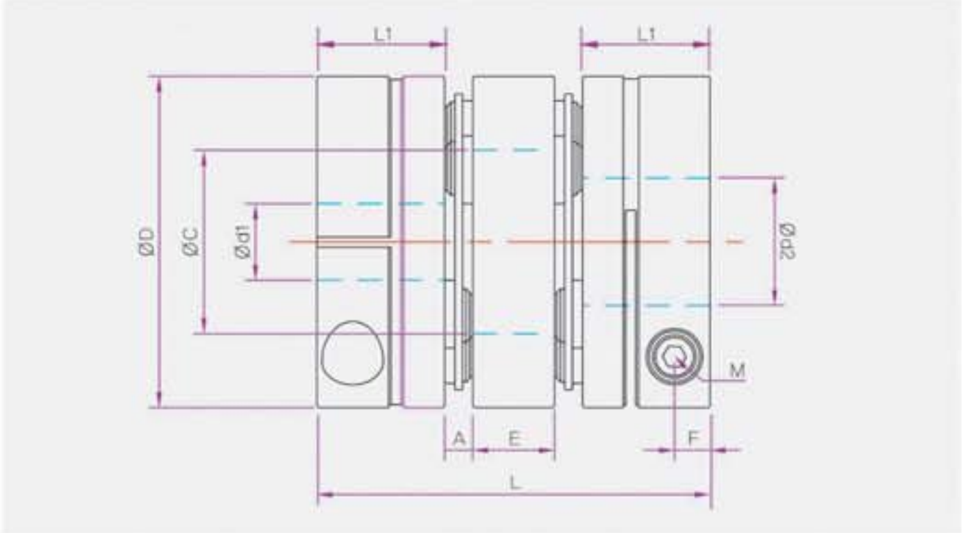
SHDW - ■■C (CLAMP TYPE)
