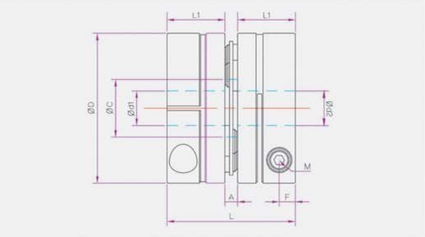
SHDS - ■■C (CLAMP TYPE)
