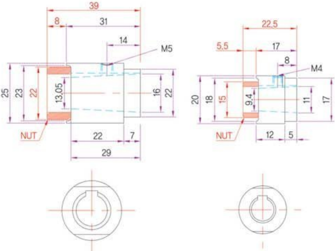
1/10 Taper Bushing
